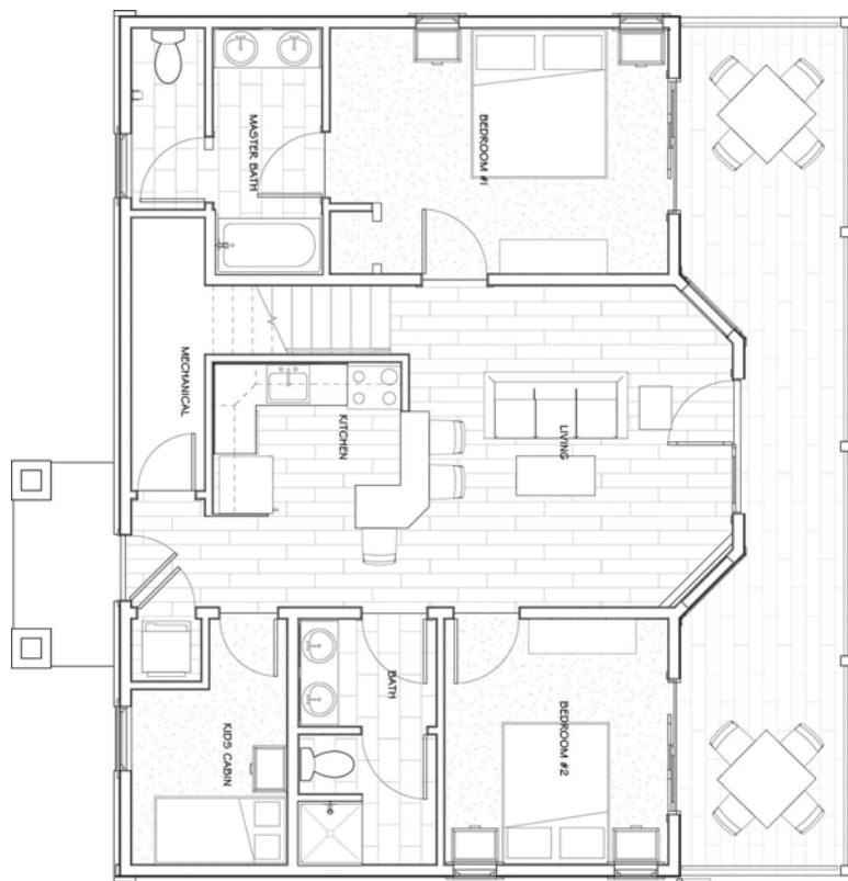
4 BEDROOM CABIN FLOOR PLAN
