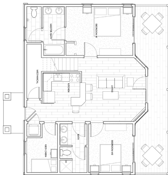
4-BEDROOM CABIN FLOOR PLAN
