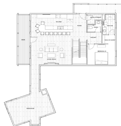
TREEHOUSE CABIN FLOOR PLAN, Lower Floor
